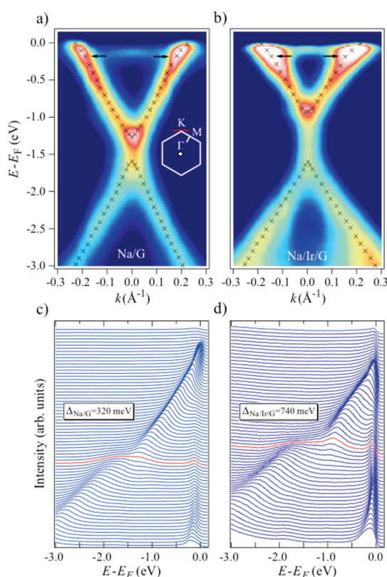
Figure 2. (a) ARPES map along the \pi\Gamma K direction for Na/G and (b) Na/Ir/G. The inset shows the 2D Brillouin zone of graphene. The red line indicates the \pi\Gamma K direction. Black crosses overlaid to the ARPES maps mark the maximum of the photoemission spectral-weight intensity, whereas arrows highlight kinks in the electronic band dispersion. (c) EDCs along the \Gamma K direction from k = 1.4 \text{ \AA}^{-1} (bottom) to k = 2.2 \text{ \AA}^{-1} (top) for Na/G and (d) Na/Ir/G. Red curves are measured at the K -point.
